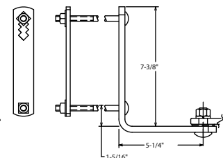
OPTION "X" EXTENDED BRACKET
